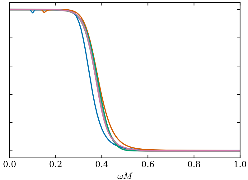
even parity, \ell = 2 (even: model C)
