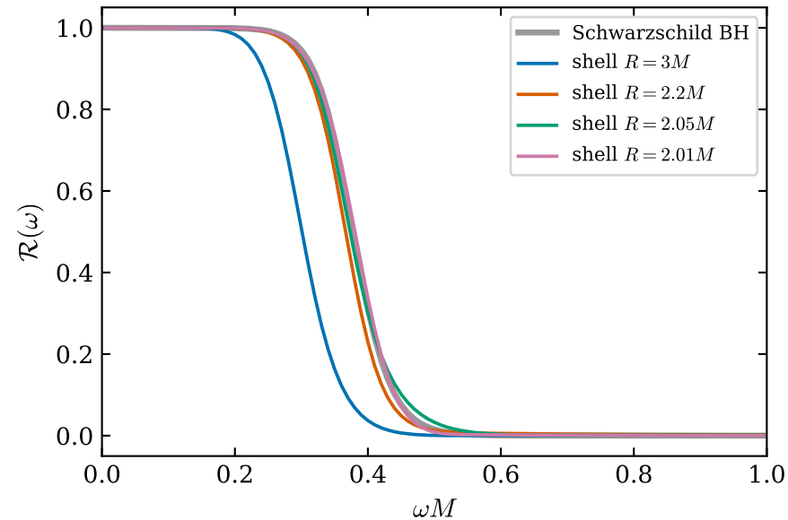
odd parity, \ell = 2 (even: model C)
